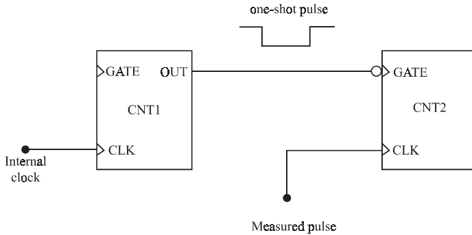
Figure 5-6: Frequency measurement
