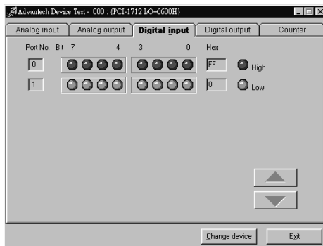
Figure 2-12: Digital Input tab on the Device Test dialog box
