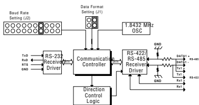
ADAM-4520 Converter Function Diagram
