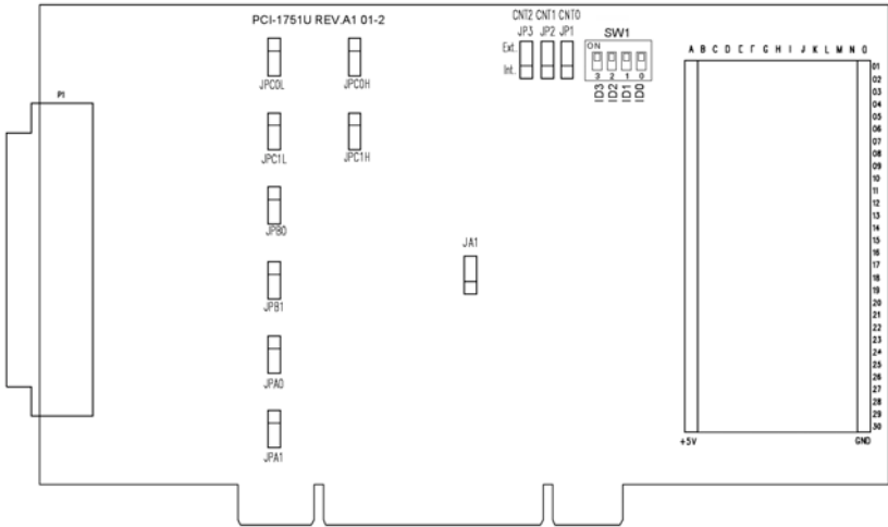
Figure 2.1: Location of Connectors and Jumpers
