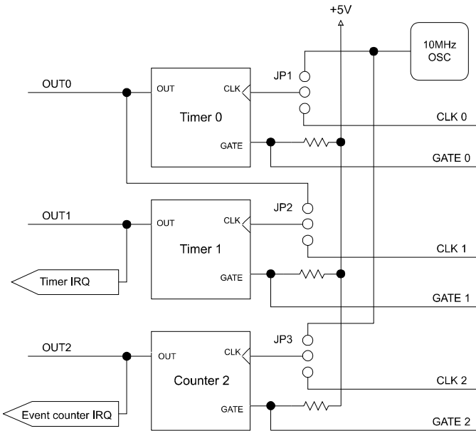
Figure 3.2: Timer and counter structure
