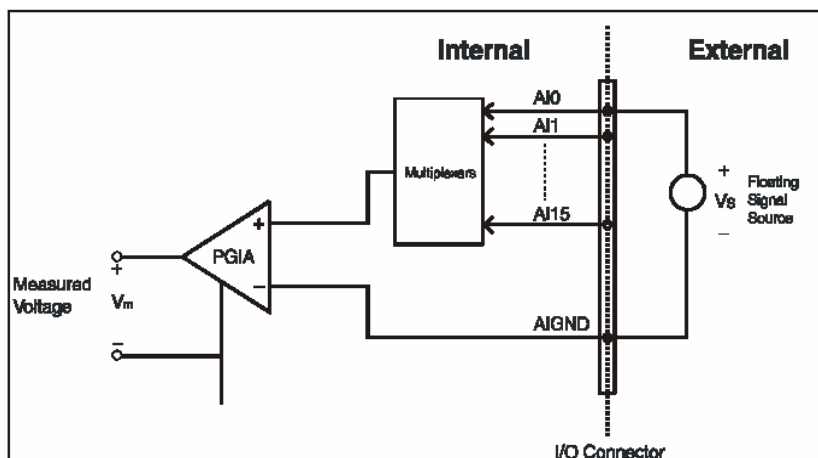
Fig. 3-2 Single-ended input channel connection
