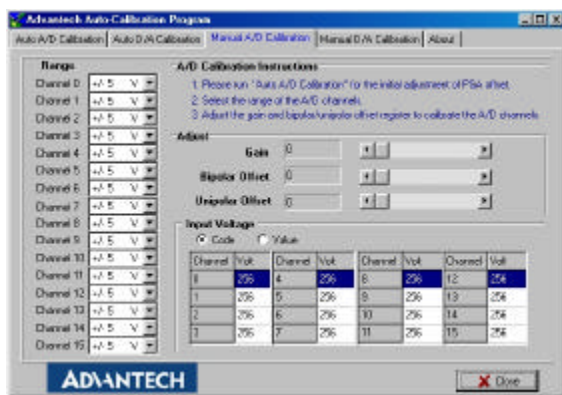
Fig. 5-16 Adjusting registers
