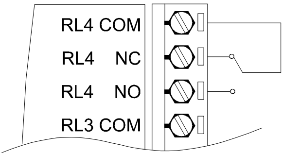
Figure 3-64 ADAM-4060 Form C Relay Output Wiring Diagram
