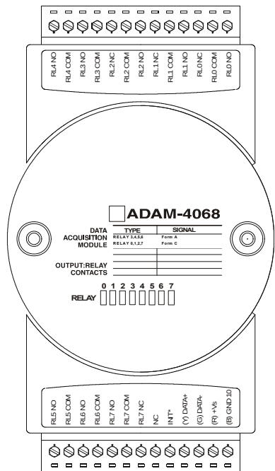
Figure 3-62 ADAM-4068 8-channel Relay Output Module
